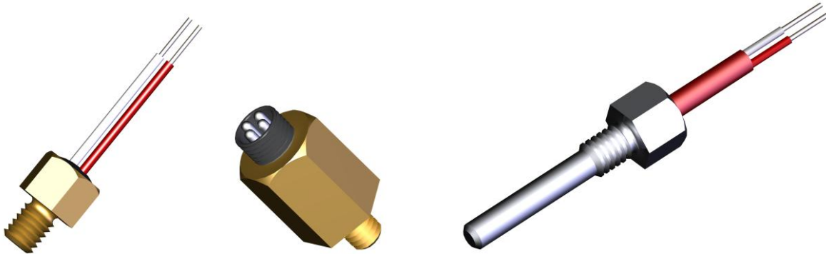
Fig. 18: Left: XXX-SGH construction A with PTFE single strands Middle: XXX-SGH construction A with fix shed connector Right: XXX-SGH construction B with silicone insulated hose liner
